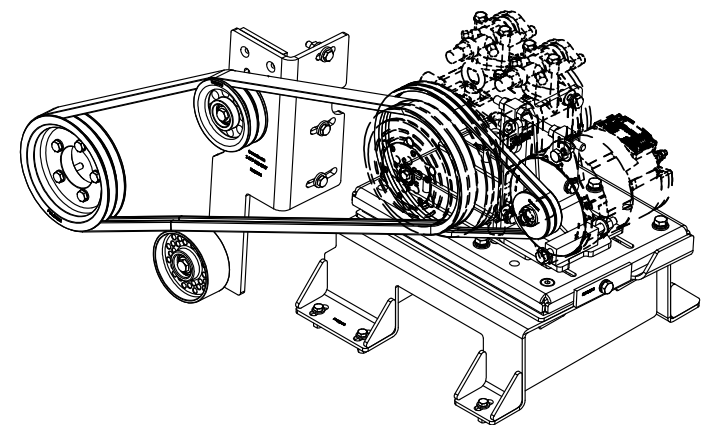
ISOMETRIC VIEW
