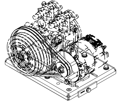
ISOMETRIC VIEW
