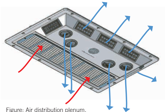
Figure: Air distribution plenum.
