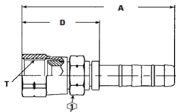
Female SAE 45° Flares
