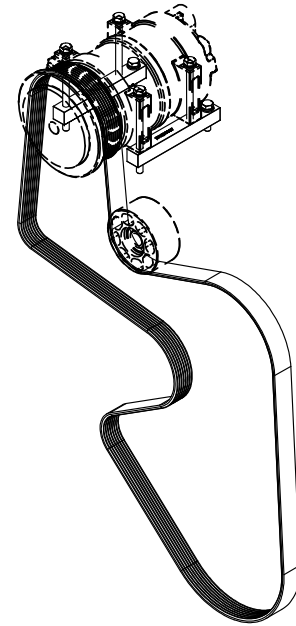
ISOMETRIC VIEW
