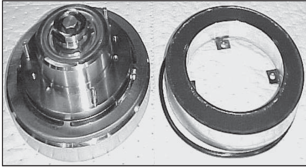
Clutch Assembly (clutch & coil) Sutrak USA P/N - 554.142 Carrier P/N - 20-554-142
