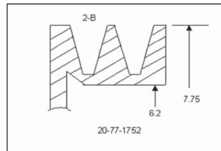
Pulley, 2-2B TK P/N 77-1752 Carrier P/N 20-77-1752
