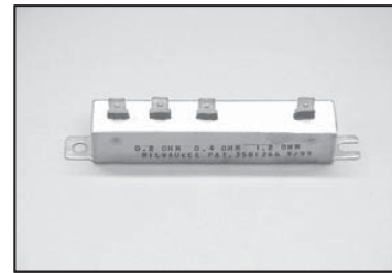
Resistor, 1.8 Ohm, 4 Tap Transair P/N 111060 Carrier P/N AC201-611
