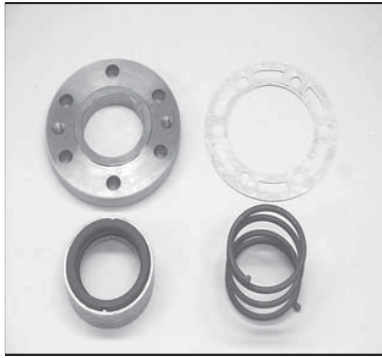
Shaft Seal, Bock FK4 Sutrak P/N 8005 Carrier P/N 24-01-75-105
