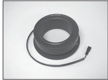
24V Clutch Coil TK P/N 45-271 Carrier P/N 20-45-271
