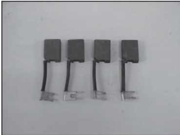
Brush Set, GE Motors TK P/N 44-5416 Carrier P/N 20-44-5416
