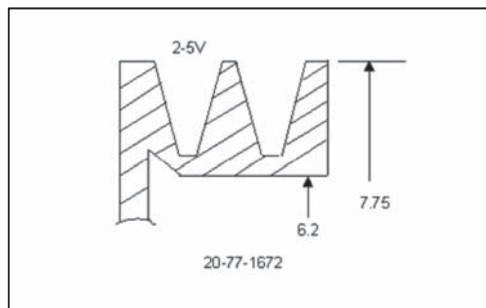
Pulley, 2-5V TK P/N 77-1672 Carrier P/N 20-77-1672
