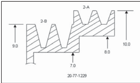
Pulley, 2-B / 2-A TK P/N 77-1229 Carrier P/N 20-77-1229
