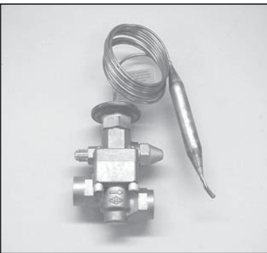
TXV, R22 Sutrak P/N 528.123 Carrier P/N 24-04-01-087
