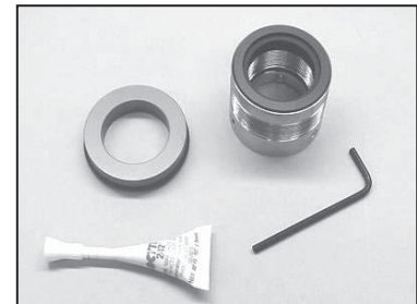
Shaft Seals, Metal Bellows TK P/N 22-751 Carrier P/N 20-22-751 TK P/N 22-1100 Carrier P/N 20-22-1100
