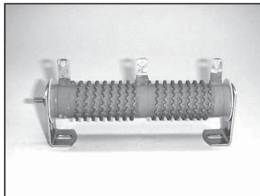
Resistor, .9 Ohm Fixed TK P/N 44-6348 Carrier P/N 20-44-6348
