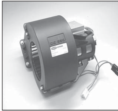
Blower Assy, w/Speed Control Sutrak P/N 735.019BLOW Carrier P/N 28-20-01-016
