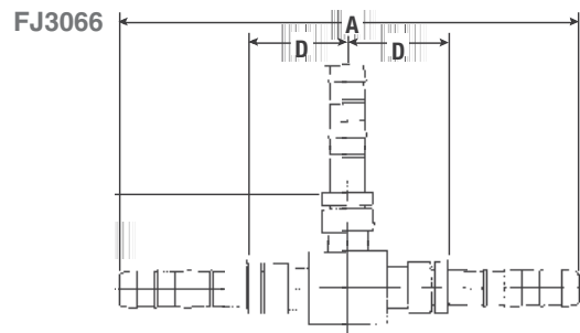
"T" Splicer – 3 Hose Connector
