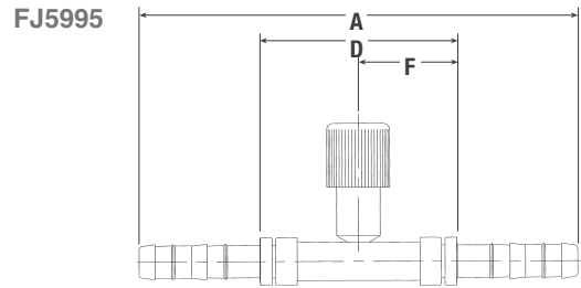
Splicer with High Side R134a Port
