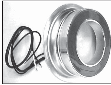
24V Coil, Vapor/TK Vapor P/N COL-2126 TK P/N 304-272 Carrier P/N 20-304-272
