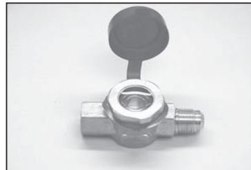
Sight Glass Transair P/N 211004 Carrier P/N AC101-200
