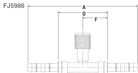
Splicer with R134a Low Side Port
