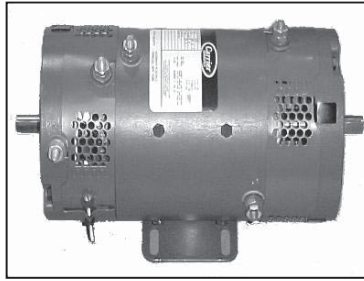
DC Motor, Evaporator TK P/N 104-651 Carrier P/N 54-50077-00
