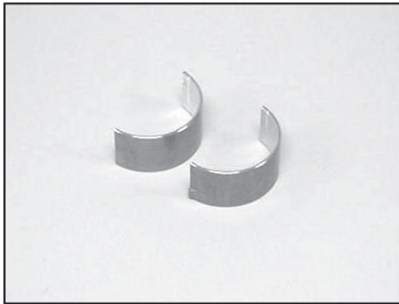
Bearings, Connecting Rod Standard - P/N 20-22-1246 .010" Over P/N 20-22-1265 .020" Over P/N 20-22-1266 .030" Over P/N 20-22-1007
