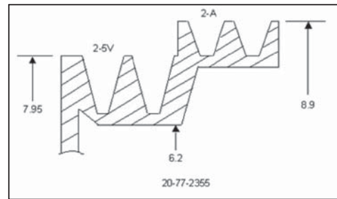
Pulley, 2-5V / 2-2A TK P/N 77-2355 Carrier P/N 20-77-2355
