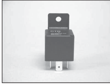
Relay TK P/N 44-9111 Carrier P/N 10-00286-03
