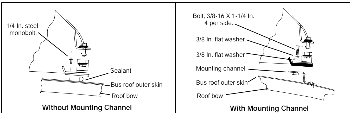
Figure 3-14 Mounting Options
