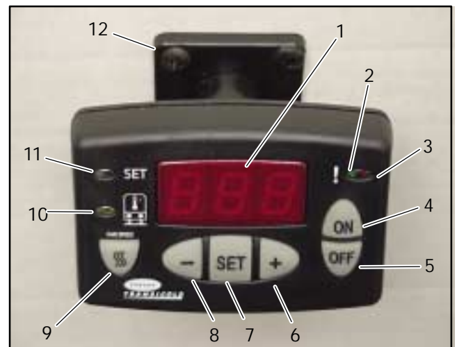
Figure 5-6 Drivers Control Panel (Dual Systems)
