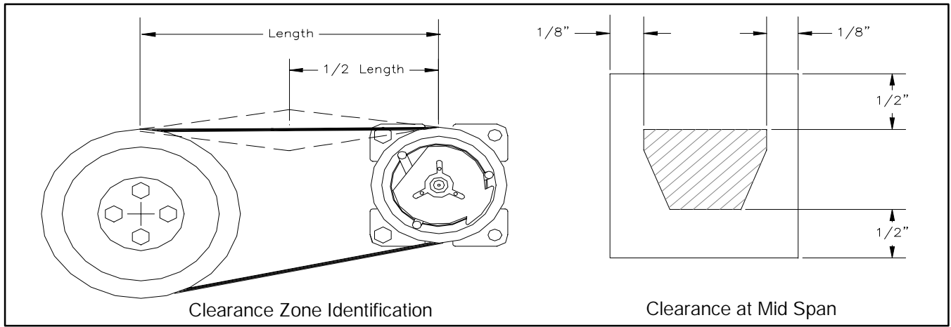
Figure 6-5 Belt Clearance Requirements
