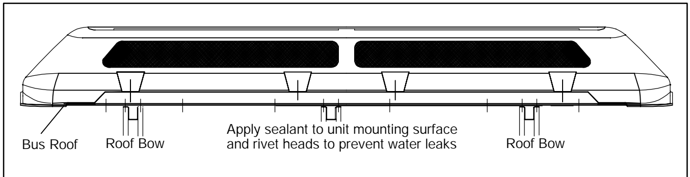
Figure 3-17 Condenser Mounted Without Mounting Channels (Side View)
