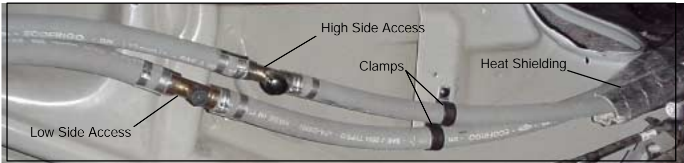
Figure 4-21 Hose Routing - OEM (To & From Engine)
