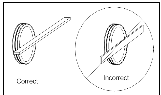
Figure 6-7 Straight-Edge Application
