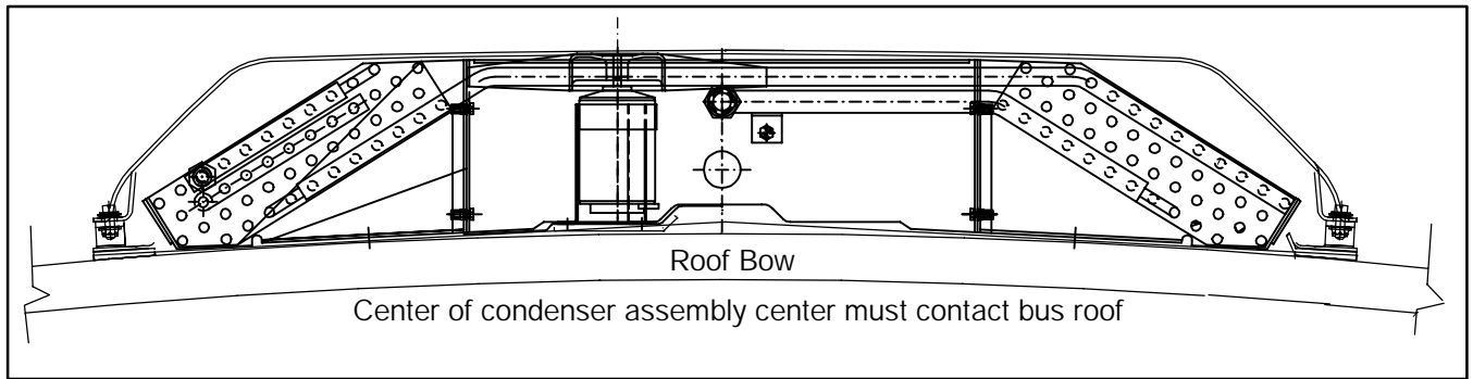
Figure 3-15 Condenser Mounted Without Mounting Channels
