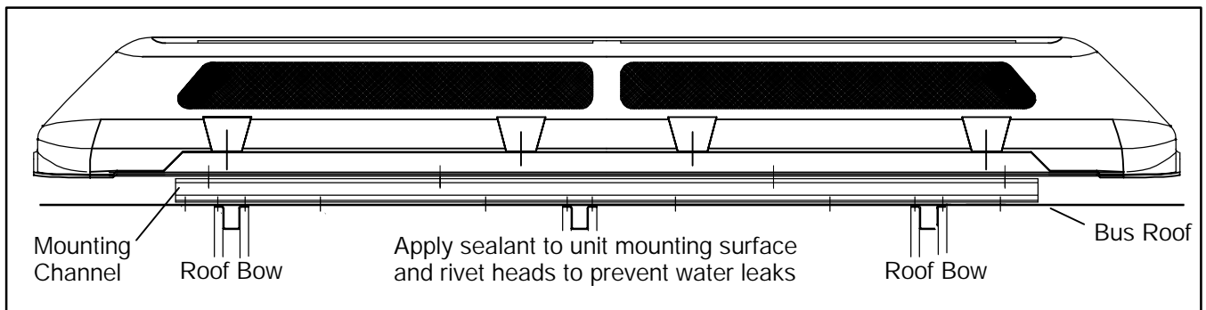
Figure 3-18 Condenser Mounted With Mounting Channels (Side View)
