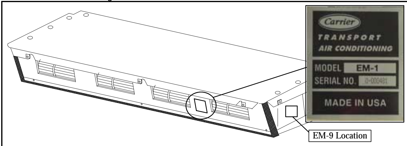
Figure 1-2 GEN 4 Evaporator Model - Serial Number Location
