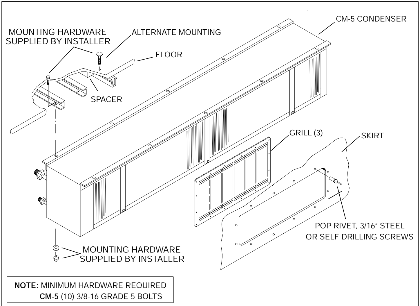
Figure 3-7 CM-5 Installation Drawing
