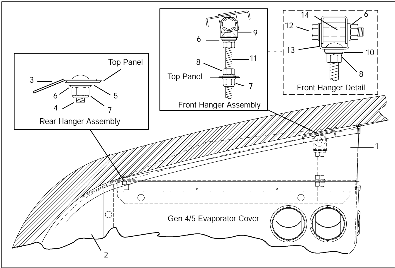
Figure 2-23 Side Mount Installation Instructions (Typical)
