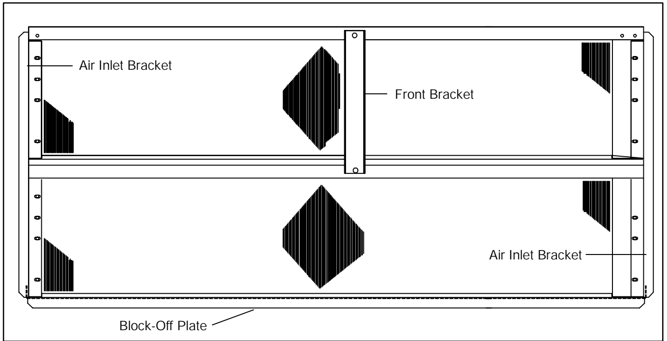
Figure 3-20 Stacked Condenser Assembly (Bus Skirt View)
