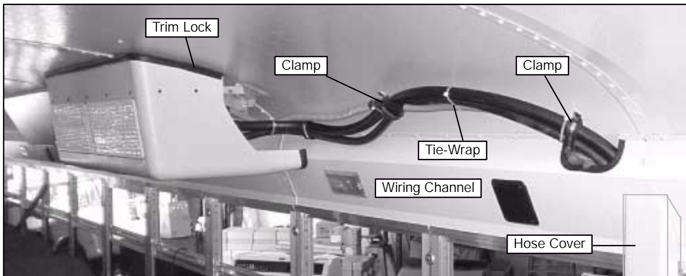
Figure 2-26 EM-9 Ducted Evaporator - Hose & Harness Routing
