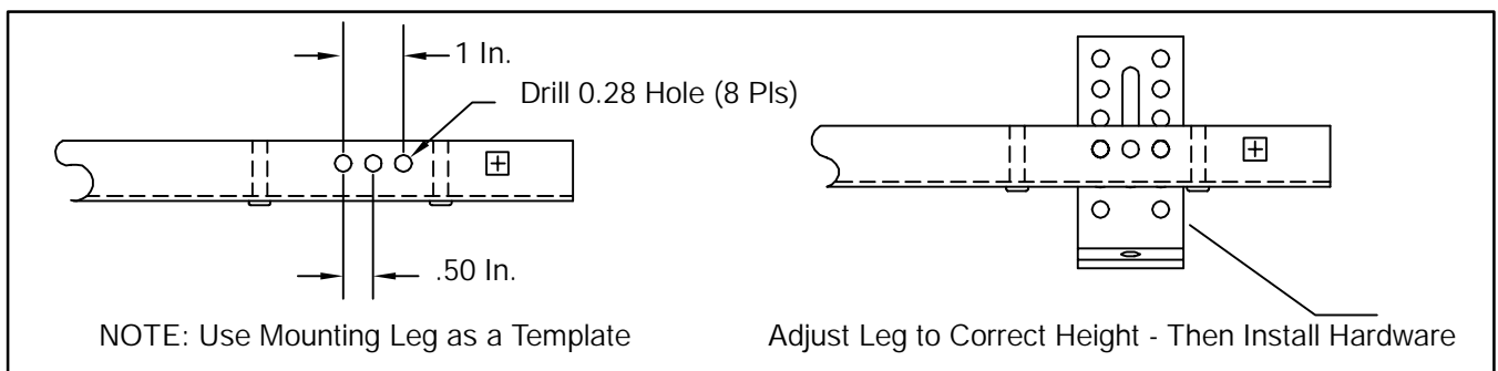
Figure 3-11 Adjusting Mounting Foot Height
