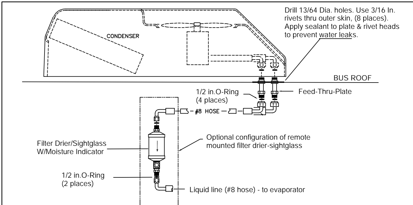
Figure 3-9 Attaching To Feed-Thru-Plate & Remote Filter Drier
