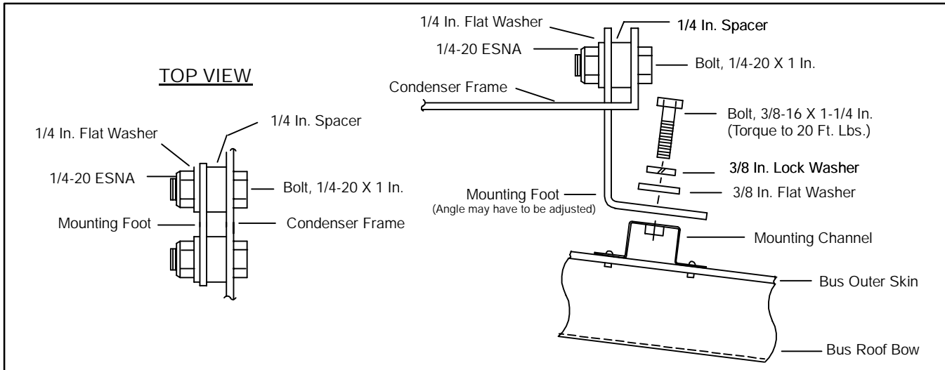
Figure 3-8 Installing Mounting Feet & Mounting Channels
