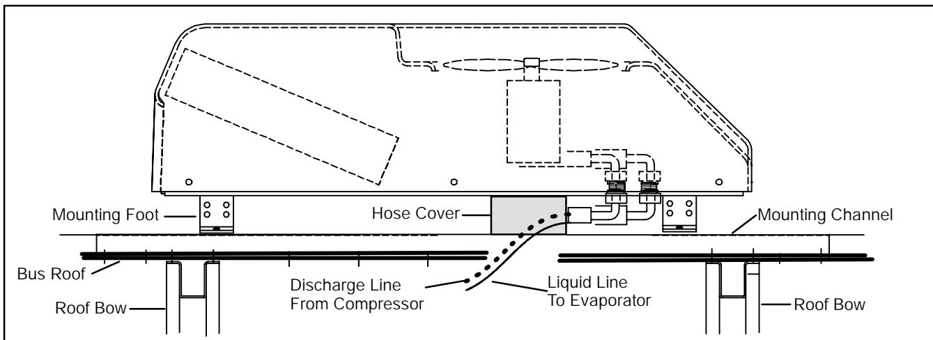
Figure 3-13 Hose Cover Transition & Refrigerant Hose Connections
