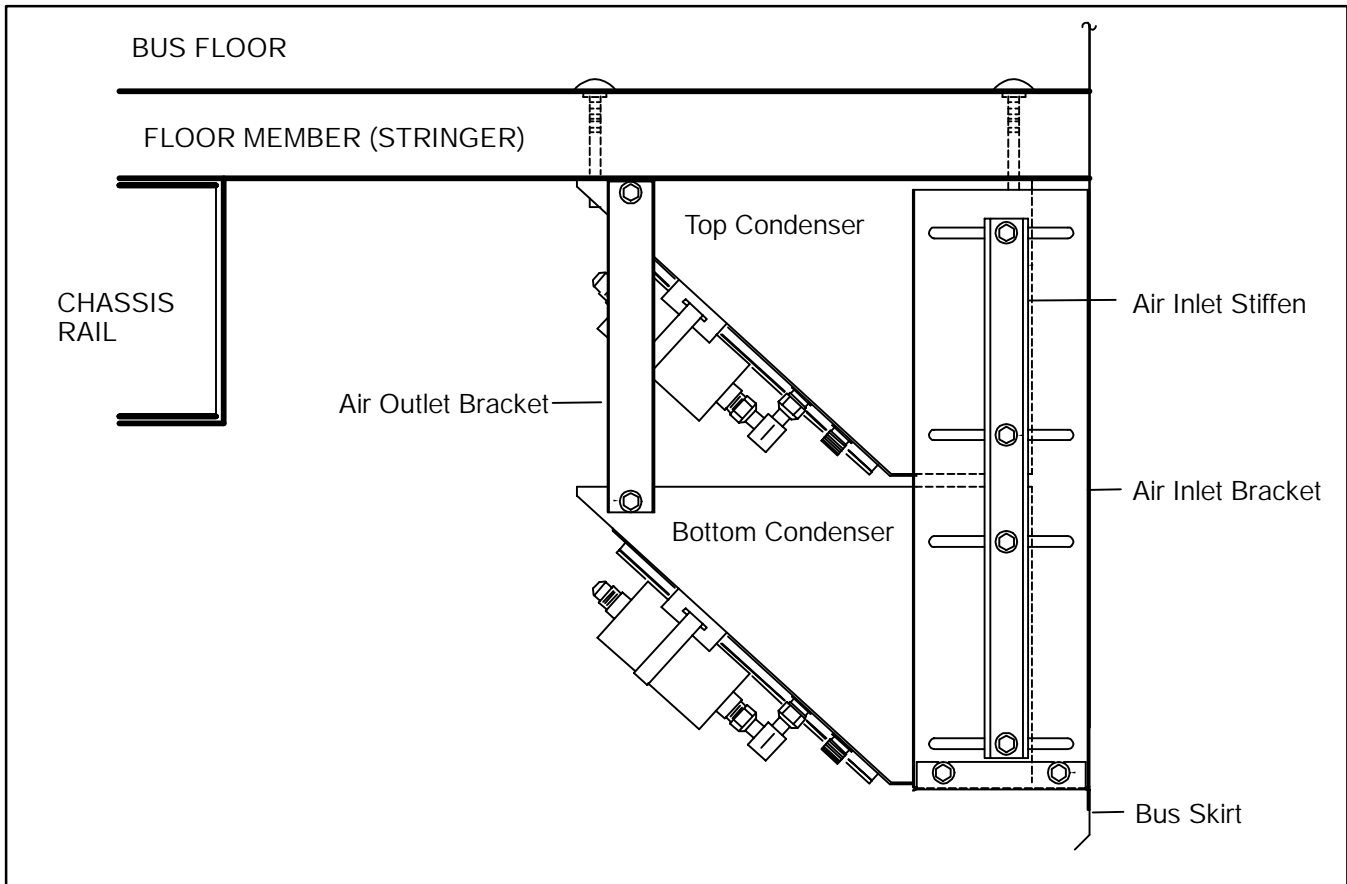
Figure 3-19 Stacked Condenser Assembly (Side View)
