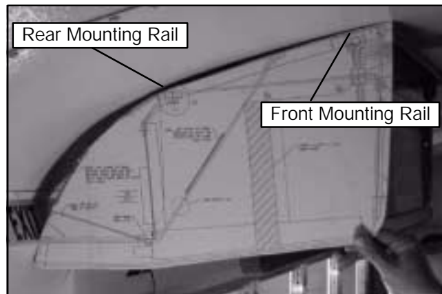
Figure 2-21 Side-Mount Template
