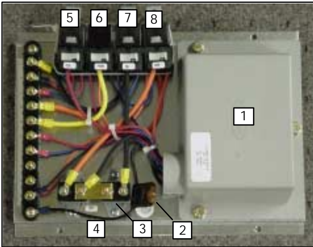
Figure 5-9 Total Control Electrical Panel (Typical)
