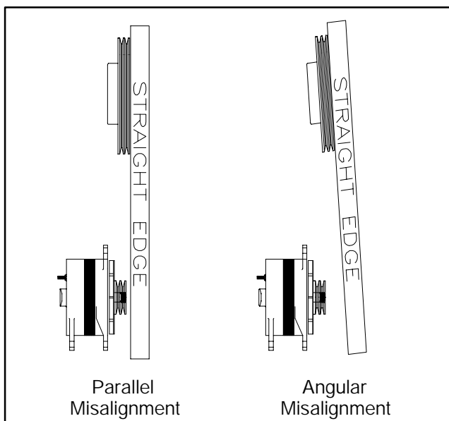
Figure 6-6 Belt Misalignment
