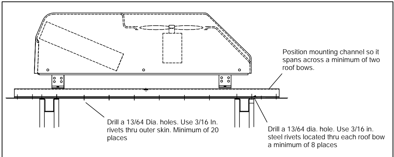
Figure 3-10 Attaching Mounting Channels To Bus Roof
