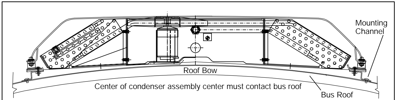
Figure 3-16 Condenser Mounted With Mounting Channels
