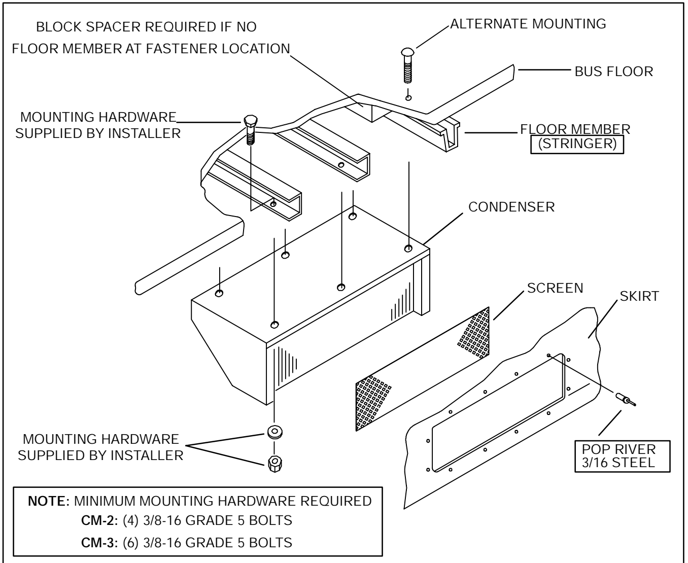
Figure 3-3 Installation Drawing (Typical Skirt Mounted)
