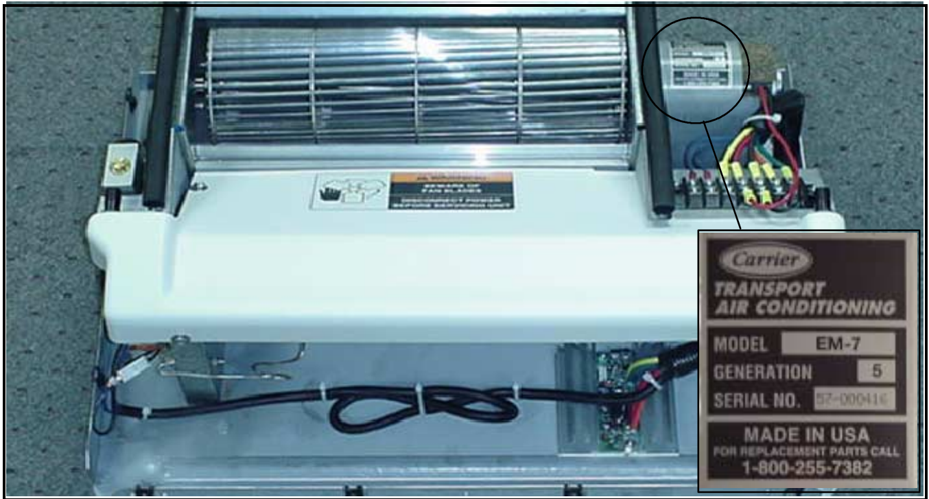
Figure 1-3 GEN 5 Evaporator Model - Serial Number Location
