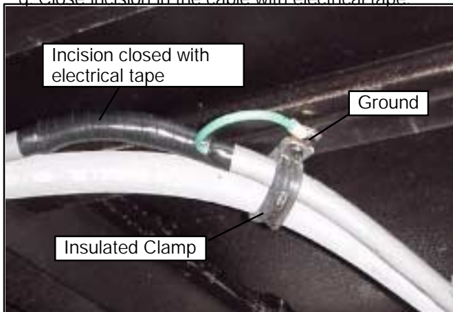
Figure 5-2 Grounded to Clamp
