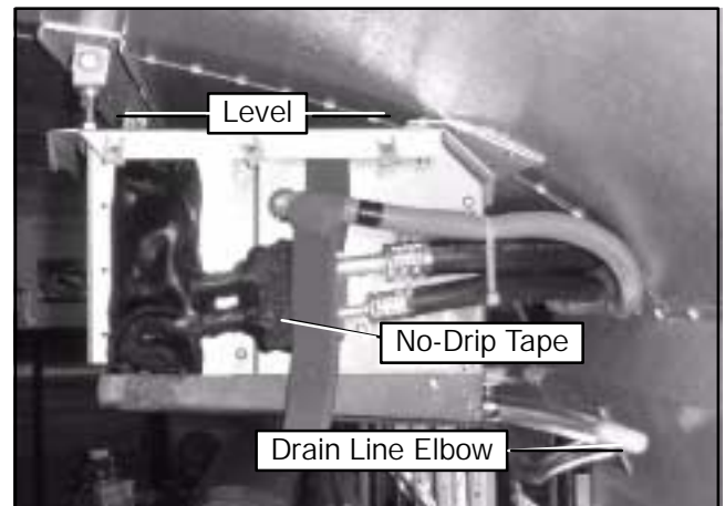
Figure 2-22 Drain Line Elbows
