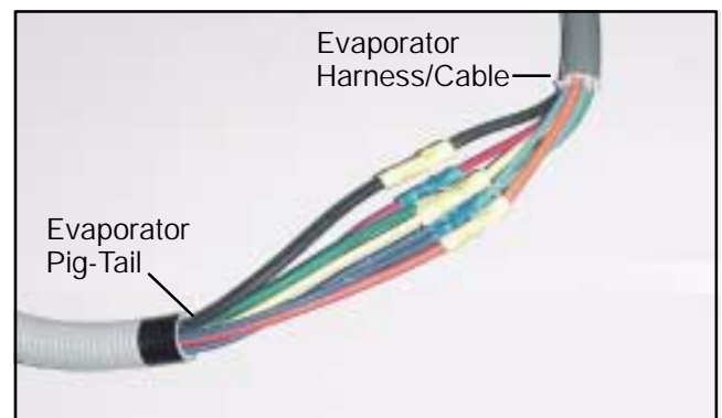
Figure 5-1 Harness & Pig-Tail Connections
